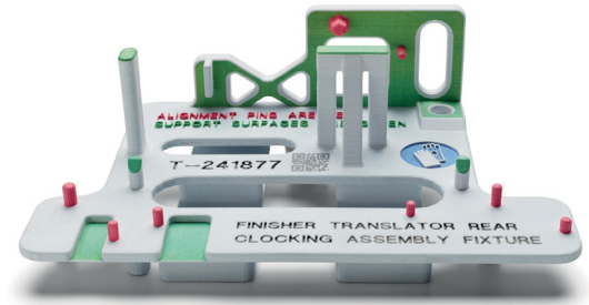
Figure 4: HP 3D HR CB PA 12 part
